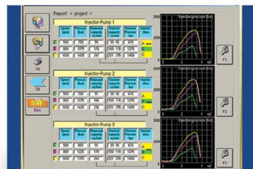
Screen shots showing individual injector pressures to monitor for internal leakage
